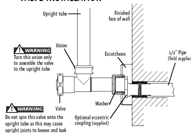
VALVE INSTALLATION
