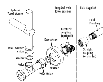
HYDRONIC HOOK-UP
